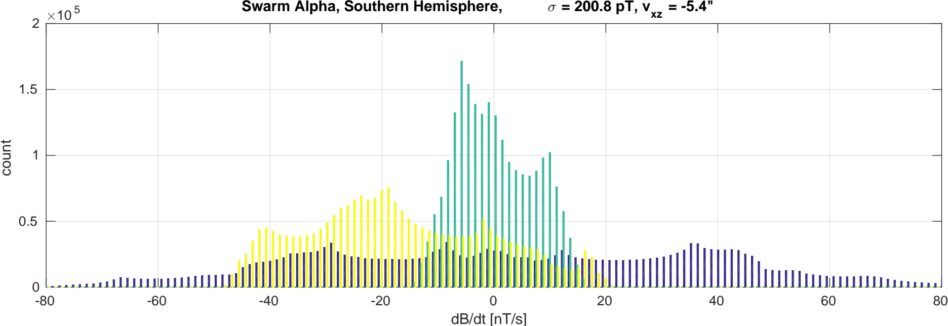
Swarm Alpha, Southern Hemisphere,
