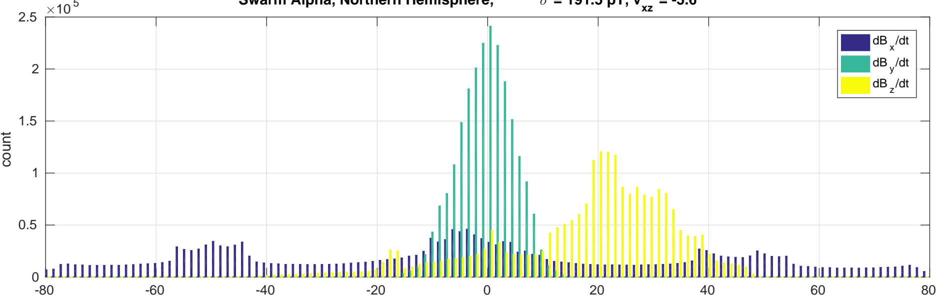
Swarm Alpha, Northern Hemisphere,
