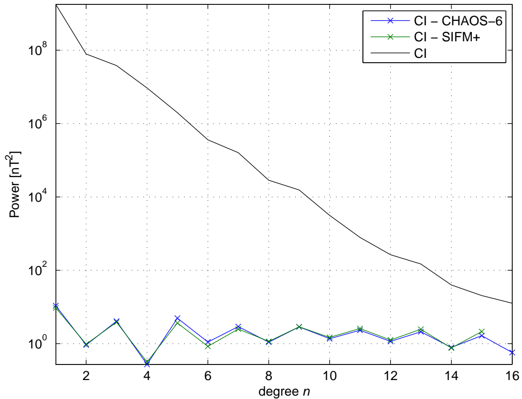
MCO Power Spectra
