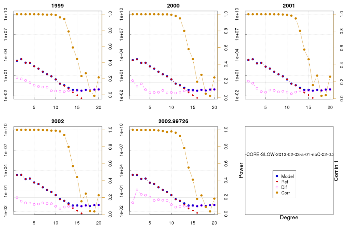
Figure 4-3: Power of difference (open circles) and correlation of evaluated model and reference model per spherical harmonic degree.
