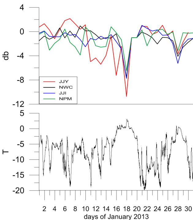
Figure 3. An example of the anomalies observed in the amplitude of the signals recorded at the PTK station during two cyclones in January 2013. The top panel shows the average residual amplitude of VLF/LF signals at nighttime, while the bottom panel refers to the temperature ( ^{\circ}\text{C} ).
