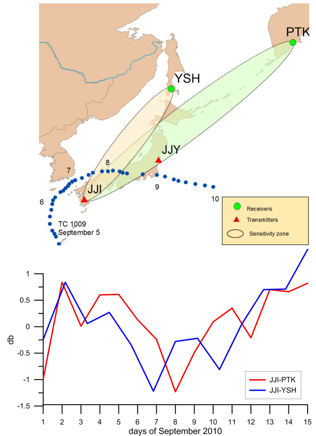
Figure 5. The anomalies in the JJI signal recorded at the PTK and YSH stations during the passage of the TC Malou (1009). Blue solid circles in the top panel show the position of the TC centres on 5–10 September 2010.
