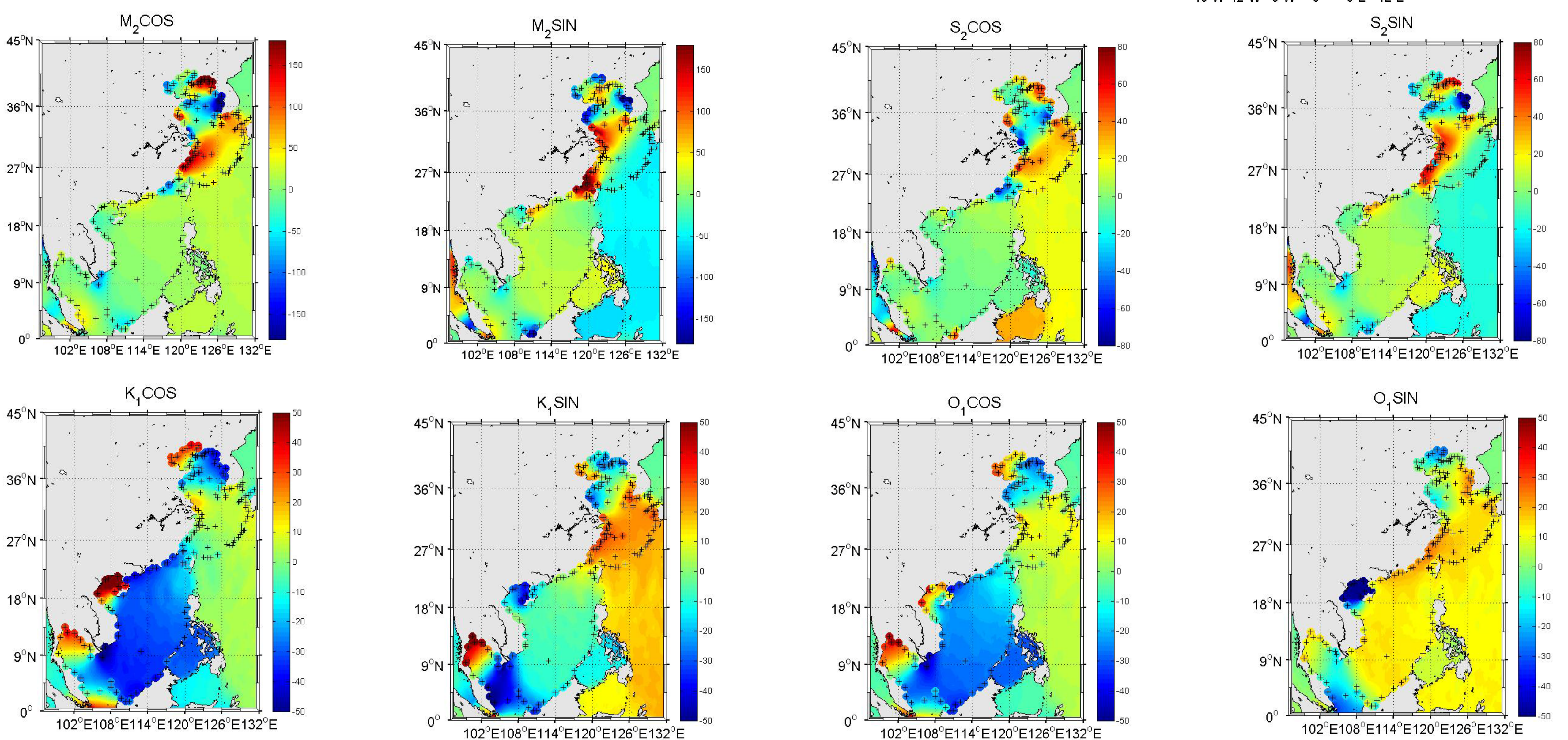
Figure 2 The real part and image part of the principle constituents from the DTU10 tide model and tide gauge measurements over the China Sea regions. The colors denote real part and image part of ocean tide solution and the reference ground truth data. The pluses denote the locations of tide gauge.
