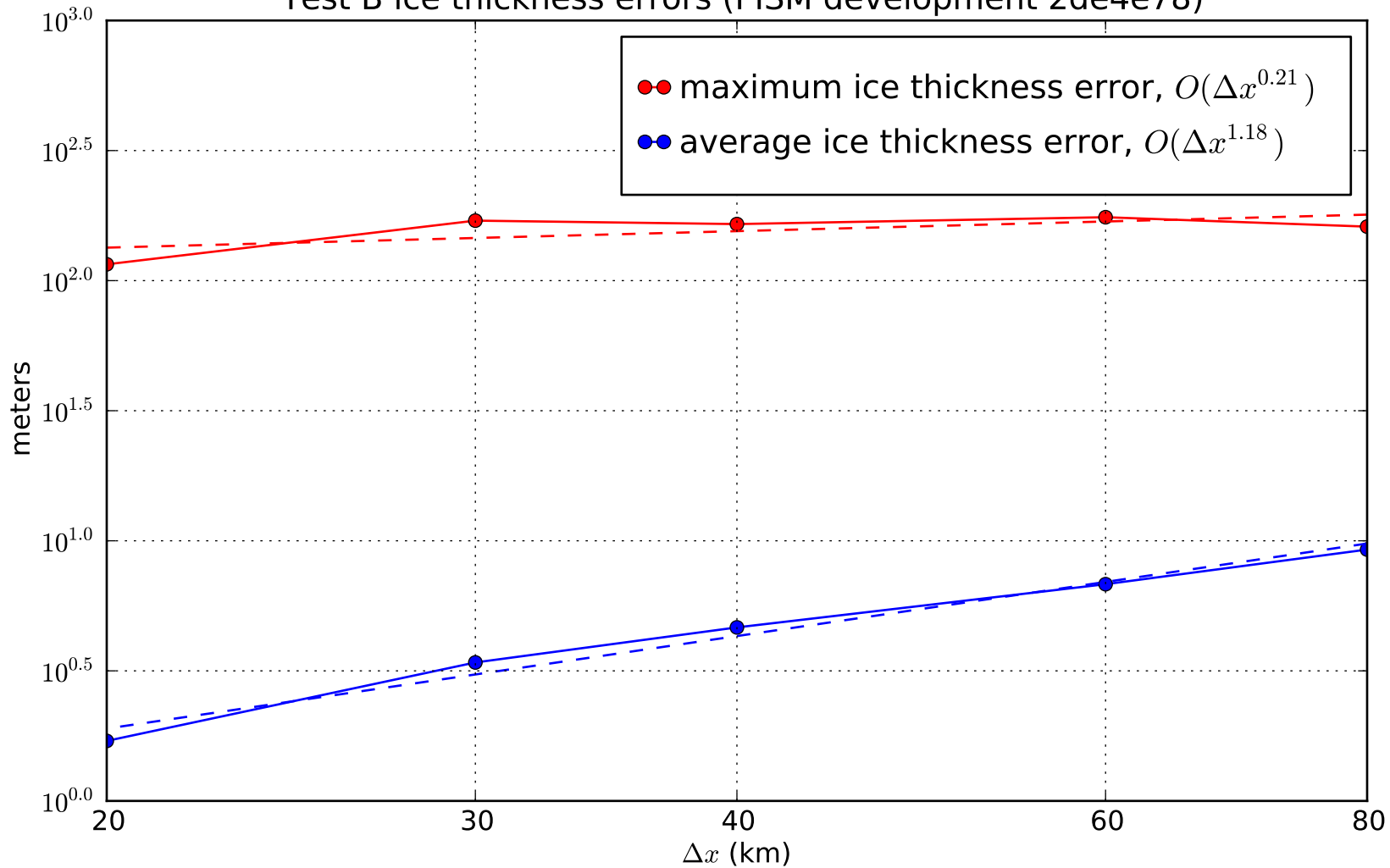
Test B ice thickness errors (PISM development 2de4e78)
