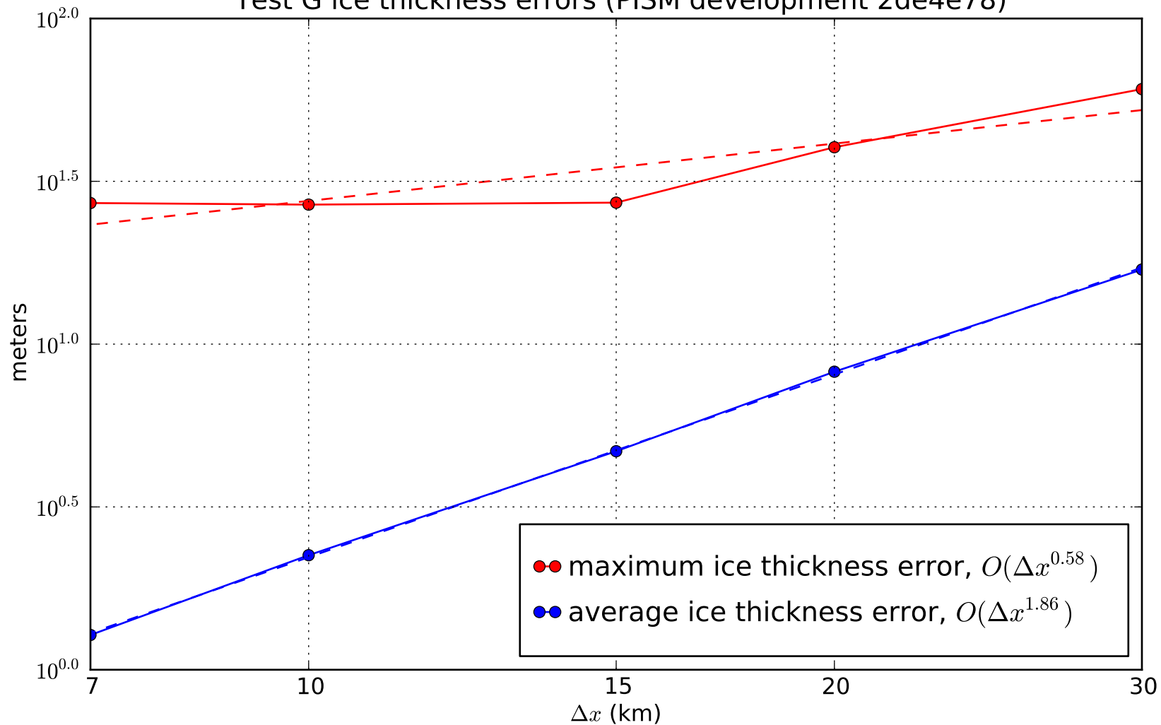
Test G ice thickness errors (PISM development 2de4e78)
