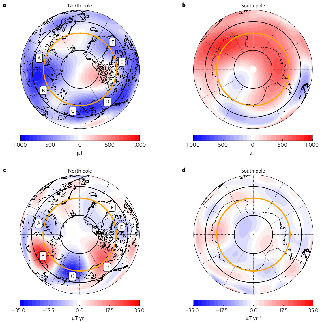
Figure 1 | Polar projection view of the radial component of the main field and secular variation at the CMB from the observation-based field reconstruction CHAOS-6 at epoch 2015. a,b, Map of the main field, to degree 13, for the Northern and Southern hemispheres, respectively. c,d, Map of the SV, to degree 16, for the Northern and Southern hemispheres, respectively. The tangent cylinder is shown in orange, and the lines of 60° and 80° latitude are shown in heavy weight. Features A-F label patches of SV of alternating sign.
