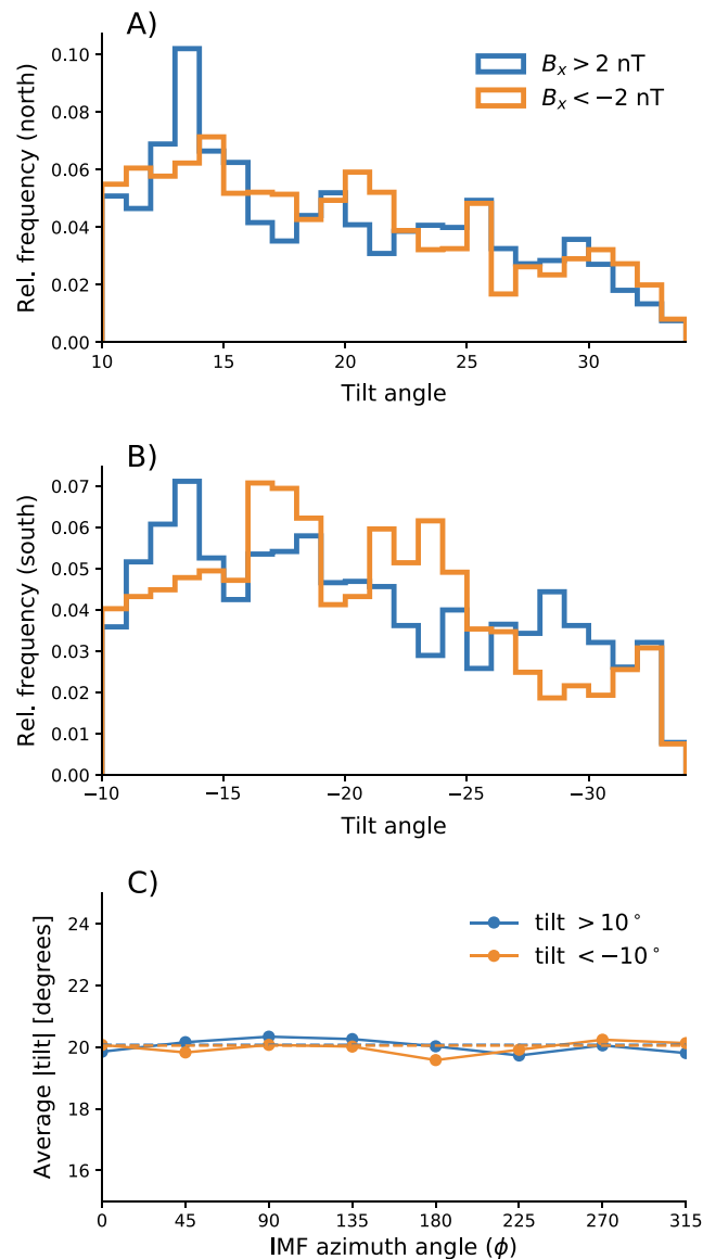
Figure A2. (a, b) Distributions of the dipole tilt angle at the times of AMPERE maps that were used to produce Figure 3. Panel (a) corresponds to maps in the Northern Hemisphere during positive tilt and panel (b) to maps in the Southern Hemisphere during negative tilt. Different colors correspond to different signs of B_x . (c) The weighted mean tilt angle in 45^\circ wide bins of interplanetary magnetic field azimuth angle, at the times of the CHAMP/Swarm data used to produce Figure 1. The weights used to calculate the means are the final Huber weights in the iterative scheme to estimate the spherical harmonic models described in section 2.1.
