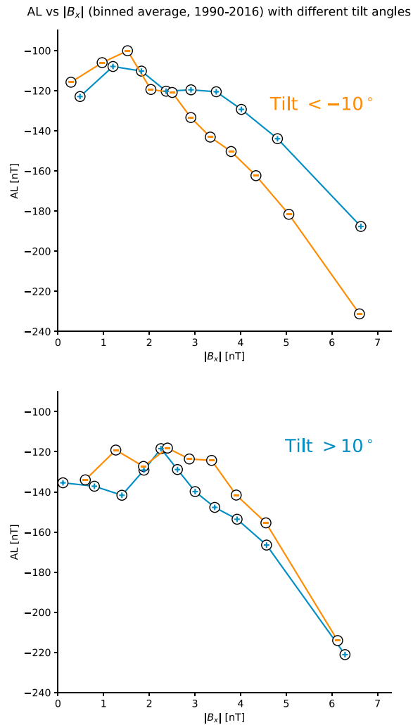
Figure 7. Average AL as a function of average |B_x| , in bins defined by quantiles of B_x during conditions defined by B_z < -1 nT, |B_y| < 1 nT, and dipole tilt < -10^\circ (top) or > 10^\circ (bottom). In each plot, the two curves correspond to different signs of B_x , with blue color indicating positive B_x and orange color indicating negative B_x . AL tends to be stronger (more negative) when B_x and dipole tilt have the same sign.
