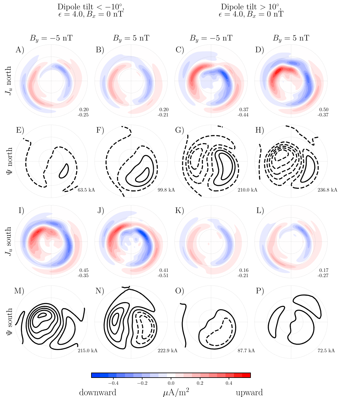
Figure B1. Same as Figure 1 but with the roles of B_x and B_y reversed.
