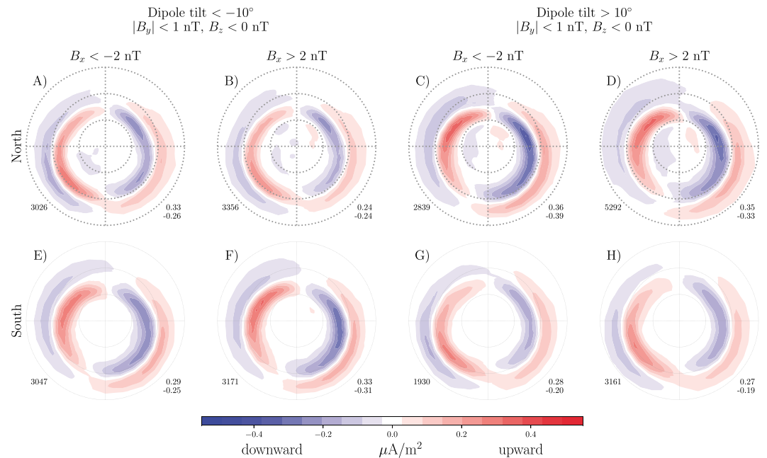
Figure 3. Maps of average AMPERE Birkeland currents from both hemispheres during B_z negative/ B_x -dominated conditions. The Northern Hemisphere is shown in the top row and the Southern Hemisphere in the bottom row. The plots in (a, e, b, f) are based on data from periods when the tilt angle was < -10^\circ , and (c, g, d, h) on periods when the tilt was > 10^\circ .
