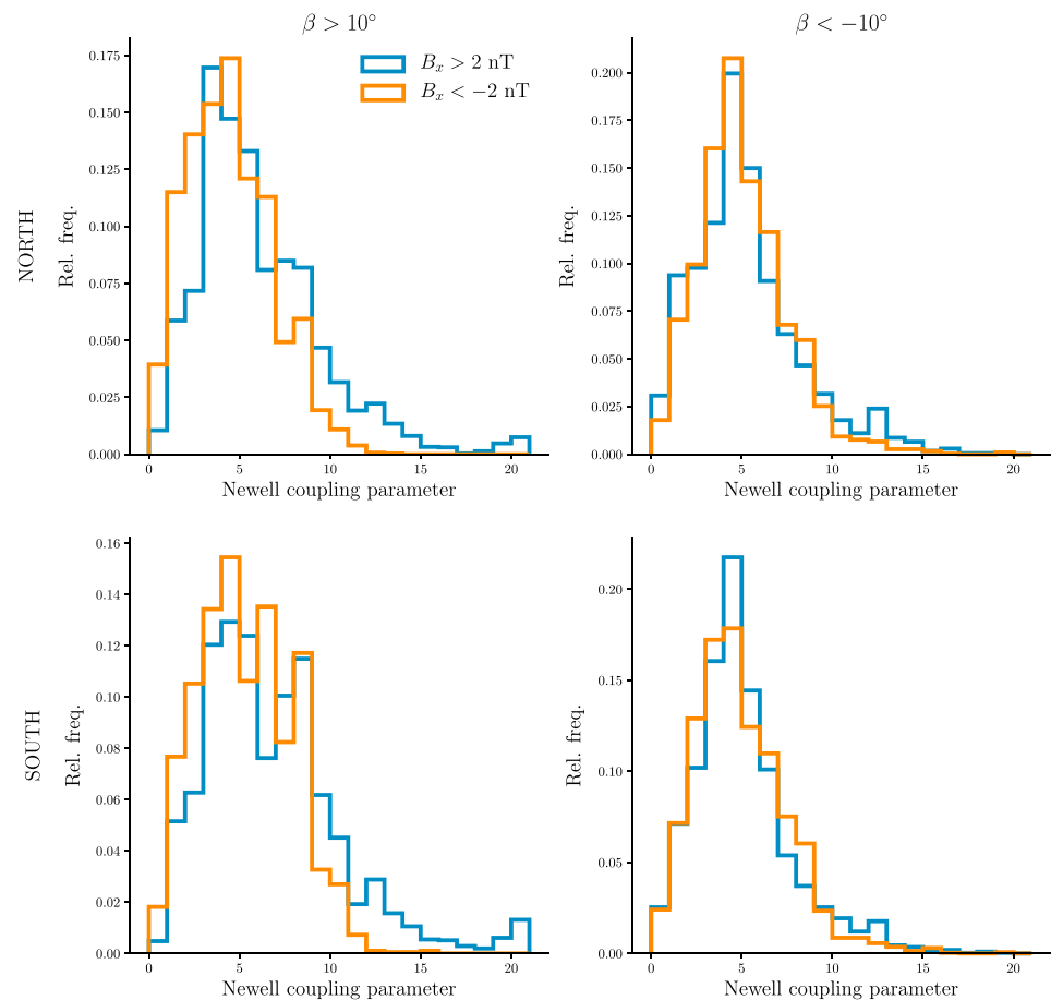
Figure A1. The distribution of Newell et al.'s, 2007 coupling parameter ( \epsilon in equation (2)) for AMPERE current maps used to make Figure (3). Each plot corresponds to one hemisphere (top row: North hemisphere, bottom row: South hemisphere) and tilt angle (left column: positive tilt, right column: negative tilt), and the two histograms in each plot correspond to different B_x bins (blue: B_x > 2 nT, orange: B_x < -2 nT).
