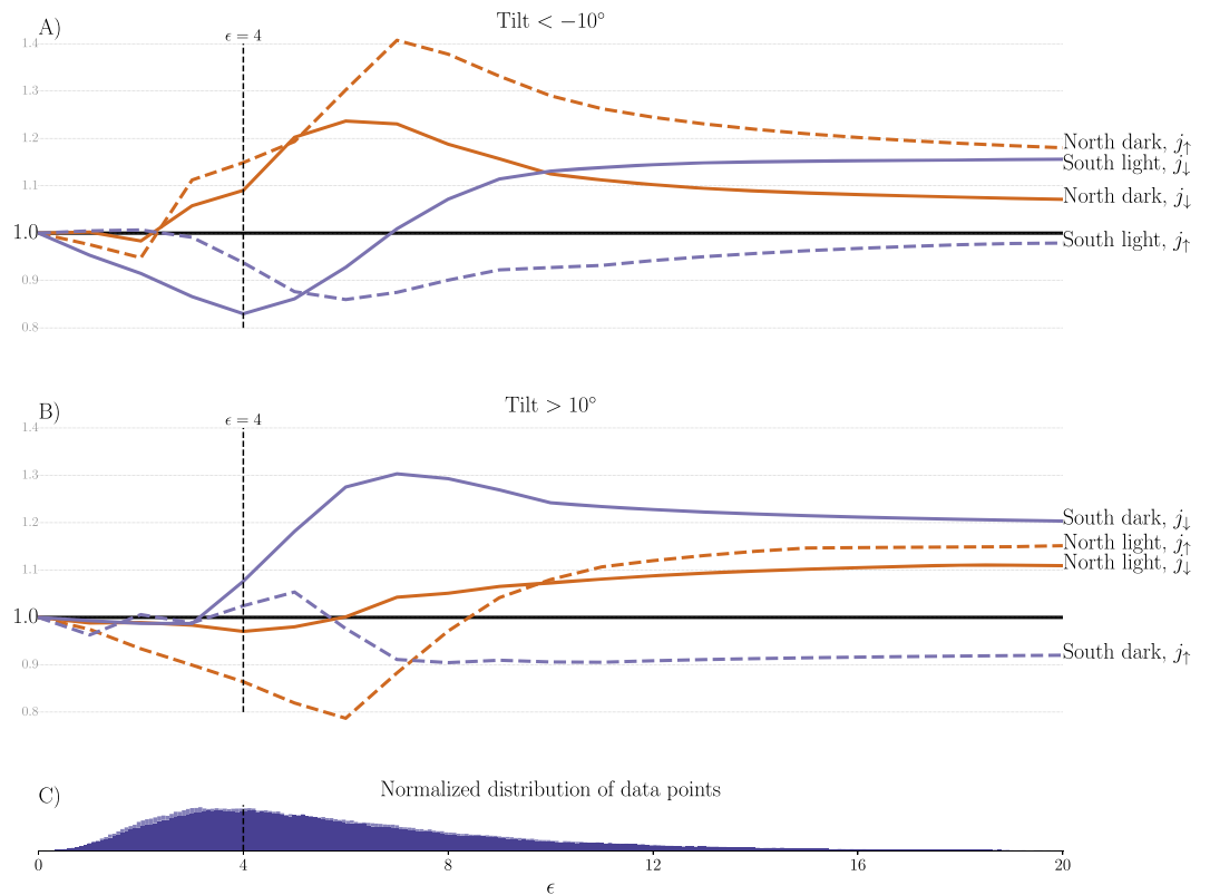
Figure 2. Ratios of corresponding R1 currents for different signs of B_x , as a function of \epsilon . The ratios are defined such that they are > 1 if the asymmetry is consistent with the Reistad et al. (2014) predictions. The curves for the two models are shown separately in (a) (tilt < -10^\circ ) and (b) (tilt > 10^\circ ). The normalized distribution of \epsilon is shown in (c). The distributions for the two models overlap where the color is dark blue.
