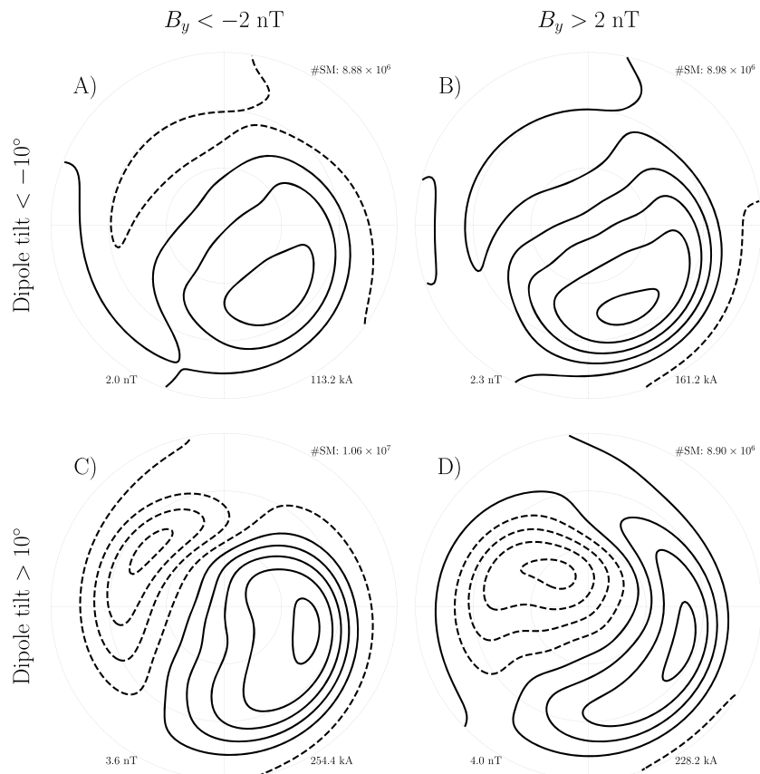
Figure B3. Same as Figure 4 but only with the roles of B_x and B_y reversed.
