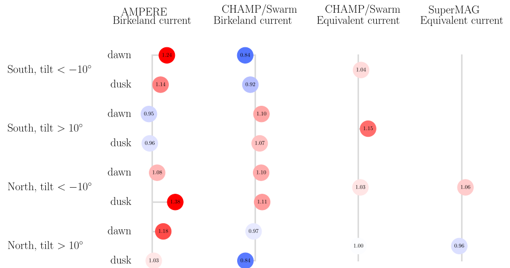
Figure 5. The ratios of corresponding currents during presumably favorable interplanetary magnetic field B_x conditions to unfavorable conditions (numbers > 1 indicate that the asymmetry is consistent with the predictions by Reistad et al., 2014). Birkeland current ratios are based on the peak values listed in Figures 1 and 3. For the equivalent currents, the ratios are based on the total current, listed in Figures 1 and 4. AMPERE = Active Magnetosphere and Planetary Electrodynamics Response Experiment; CHAMP = Challenging Minisatellite Payload.
