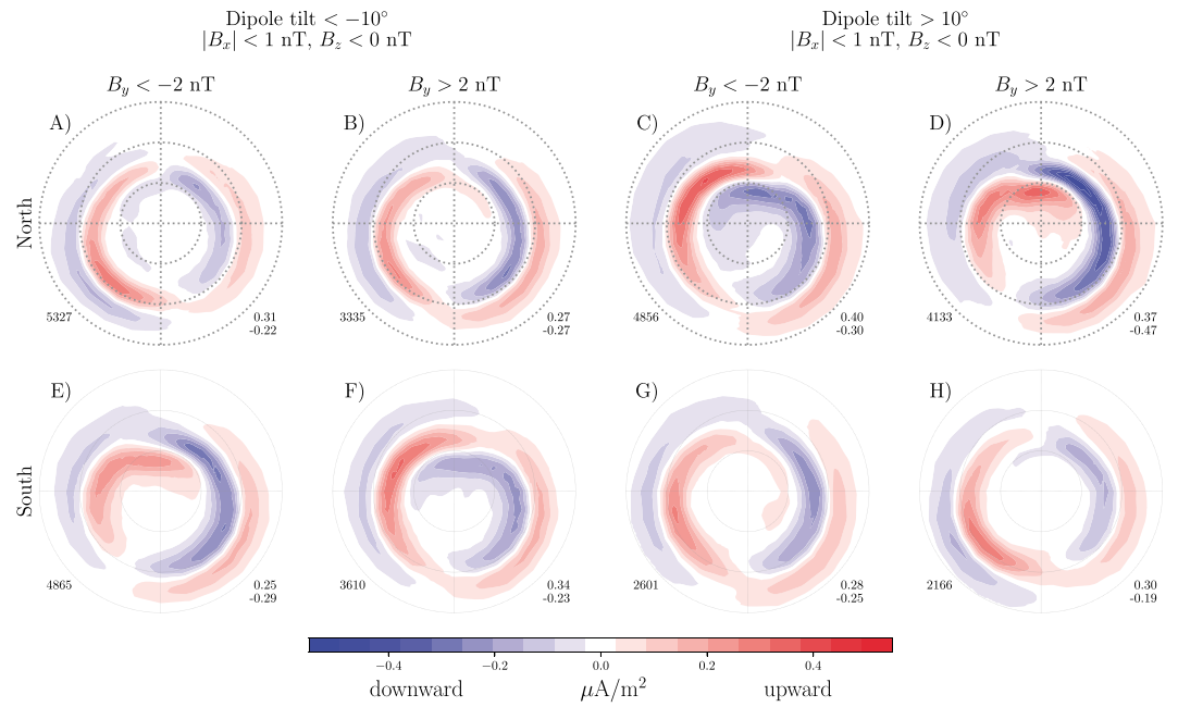
Figure B2. Same as Figure 3 but with the roles of B_x and B_y reversed.
