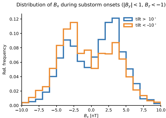
Figure 8. The distributions of interplanetary magnetic field B_x at substorm onsets that occurred when |B_y| < 1 nT, B_z < -1 nT, and the dipole tilt angle was either > 10^\circ (blue) or < -10^\circ (orange). Each histogram is based on slightly more than 1,500 onsets, from a list of more than 62,000 substorms provided by SuperMAG (1981–2015).
