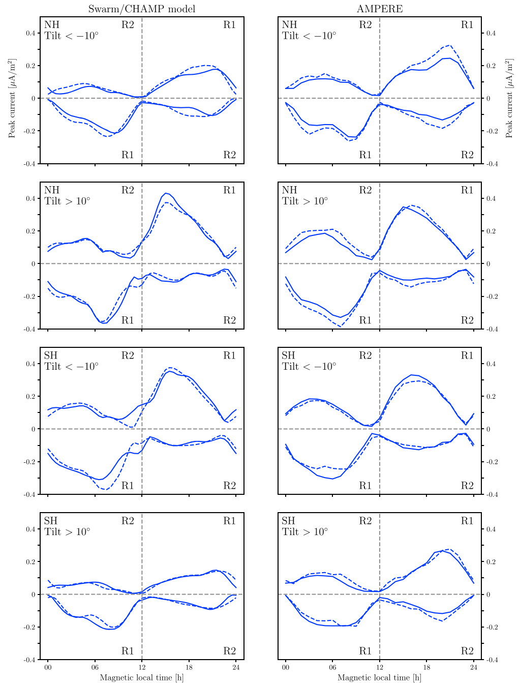
Figure 6. Peak upward and downward currents (positive and negative, respectively) as a function of magnetic local time. Blue solid curves show results for positive B_x and dashed for negative. The values in the left column correspond to the plots in Figure 1, which shows maps based on the Swarm/CHAMP models. The values in the right column correspond to the plots in Figure 3, based on Active Magnetosphere and Planetary Electrodynamics Response Experiment (AMPERE). The four quadrants are labeled by the current that contributes to the values there (R1 or R2). Tilt angle domain and hemisphere are indicated in the top left corners. NH = Northern Hemisphere; SH = Northern Hemisphere.
