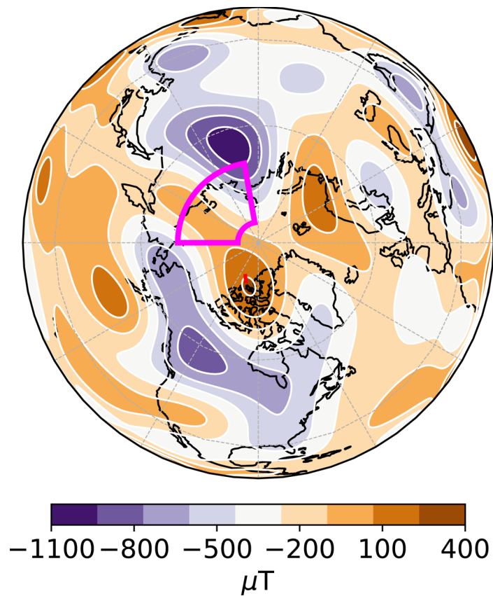
Extended Data Fig. 1 | North magnetic pole sensitivity on geomagnetic field changes beneath the New Siberian Islands. In this test, as described in the main text, between 1999–2019 the geomagnetic field on the CMB is allowed to evolve (according to CHAOS-6-x8) only within the shown wedge (centred on the New Siberian Islands). The resulting path of the north magnetic pole shows the insensitivity of the pole to secular variation restricted to this region, and is shown 1999–2019 by the red line. We have omitted to plot the red star (which is included in the other figures) since it would hide the path.
