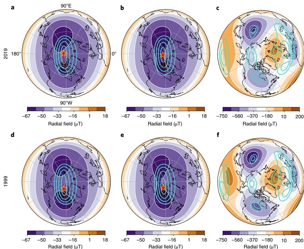
Fig. 2 | A comparison of the structure of the geomagnetic field and the north magnetic pole position in orthographic projection between 2019 and 1999. a,d , Contours of the radial field on Earth’s surface overlaid with contours of H in turquoise (values 2, 4, 6, 8 \mu\text{T} ) and the north magnetic pole as a red star with a dotted tail showing the path 1840–1999, solid tail 1999–2019. b,e , As a,d but truncated to spherical-harmonic degree 6. c,f , Structure of the geomagnetic field to degree 6 on the CMB, shown by contours of radial field overlaid with contours of H in turquoise (values 50, 100 \mu\text{T} ). In each panel lines of constant latitude and longitude are marked every 30^\circ .
