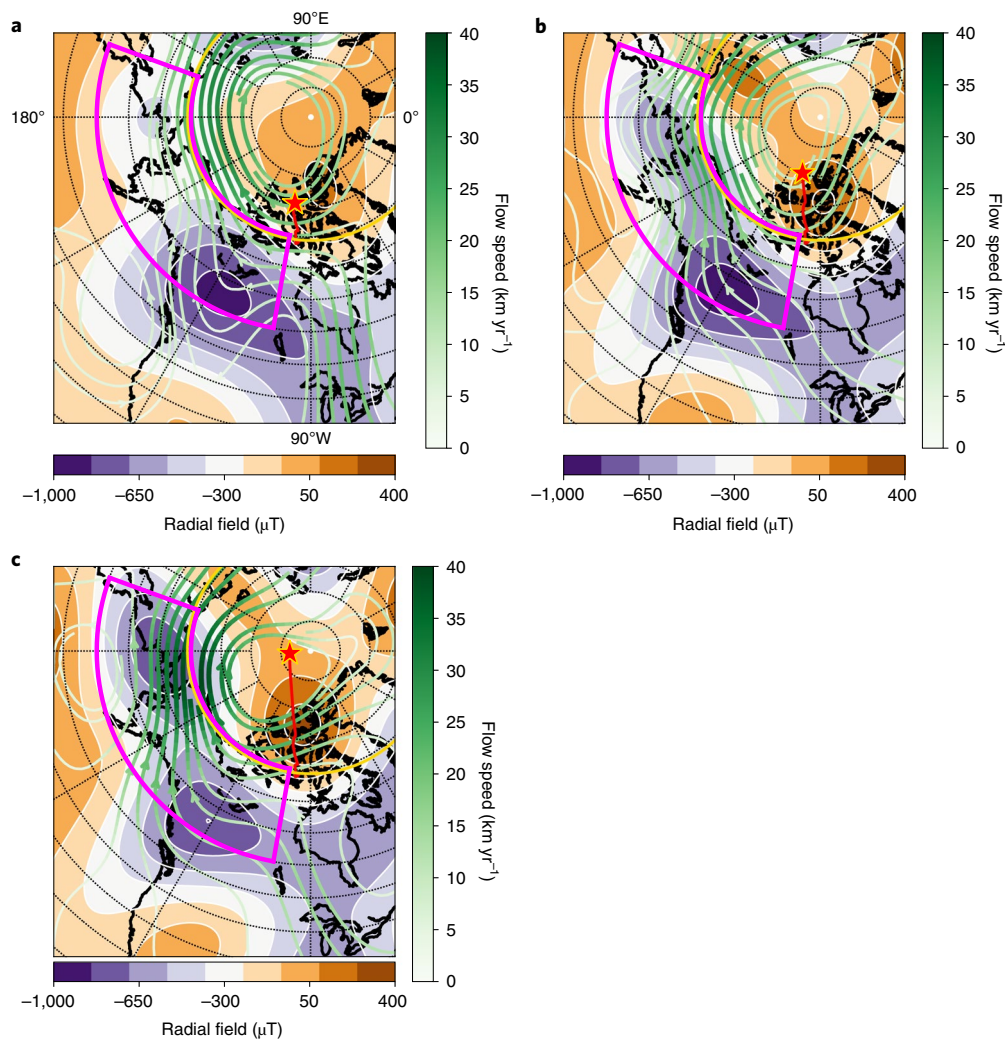
Fig. 4 | Local core surface dynamics around the Canadian flux lobe in stereographic projection. a–c, Contours of the radial magnetic field, the north magnetic pole position and path since 1840, flow streamlines with arrows and the wedge within which flux lobe elongation occurs in 1970 ( a ), 1999 ( b ) and 2017 ( c ). The 1970 magnetic field and flow data are from COV-OBS.x1 and the ensemble mean flow of refs. 19,21 ; those from 1999 are from CHAOS-6-x8 and the ensemble mean flow of refs. 19,21 ; those from 2017 are from CHAOS-6-x8 and the ensemble mean of refs. 20,21 . The inner-core tangent cylinder is marked in gold at about 69°N. In each panel lines of constant latitude are marked every 5°.
