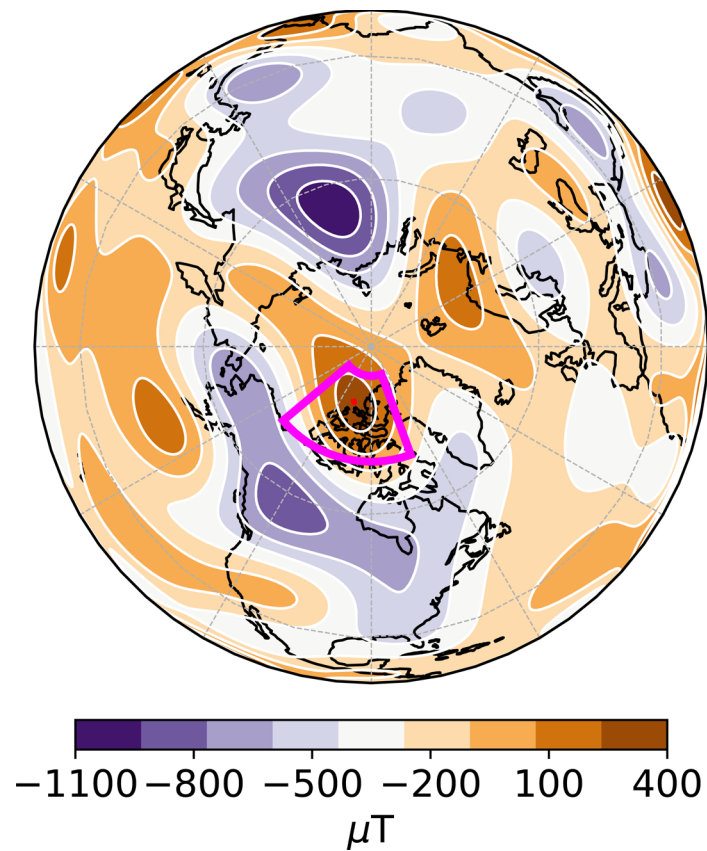
Extended Data Fig. 2 | North magnetic pole sensitivity on geomagnetic field changes beneath a high latitude reversed flux patch. In this test, as described in the main text, between 1999–2019 the geomagnetic field on the CMB is allowed to evolve (according to CHAOS-6-x8) only within the shown wedge (centred on the high latitude reversed flux patch which the north magnetic pole is currently traversing). The resulting very short path of the north magnetic pole shows the insensitivity of the pole to secular variation restricted to this region, and is shown 1999–2019 by the red line (which appears here as a single dot). We have omitted to plot the red star (which is included in the other figures) since it would hide the path.
