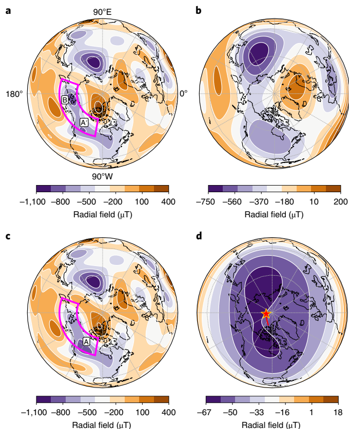
Fig. 3 | Experiment demonstrating the effect of elongation of the Canadian CMB flux lobe on the large-scale surface field and pole position. a , Radial component of a composite field projected into a divergence-free spherical-harmonic representation, comprising the structure in 2019 within the magenta wedge and the structure in 1999 elsewhere. b , Radial field on the CMB, as in a but truncated to degree 6; note that the similarity of the structure to Fig. 2c demonstrates that flux lobe elongation explains the change in the Canadian surface patch. c , Contours of the radial component in 1999 according to CHAOS-6-x8. d , Radial field on Earth’s surface with the north magnetic pole (red star), whose tail indicates its path since 1999, produced only by changes within the wedge between 1999 and 2019. In each panel lines of constant latitude and longitude are marked every 30^\circ .
