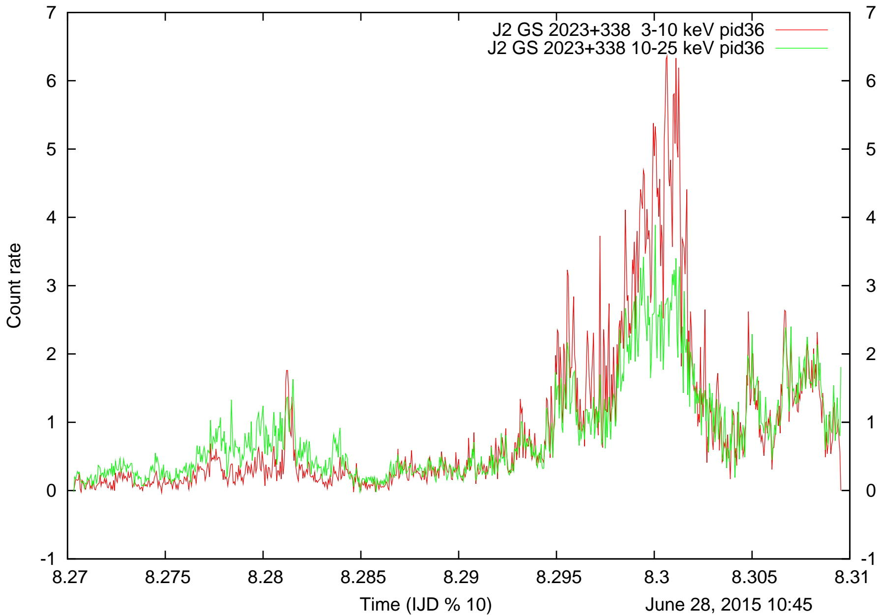
JEM X2 GS 2023+338 light curves from Rev 1554
