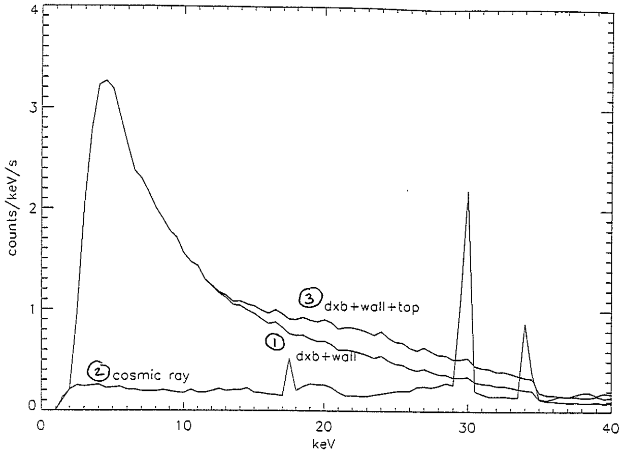
Figure 3. JEM-X Background Contributions
