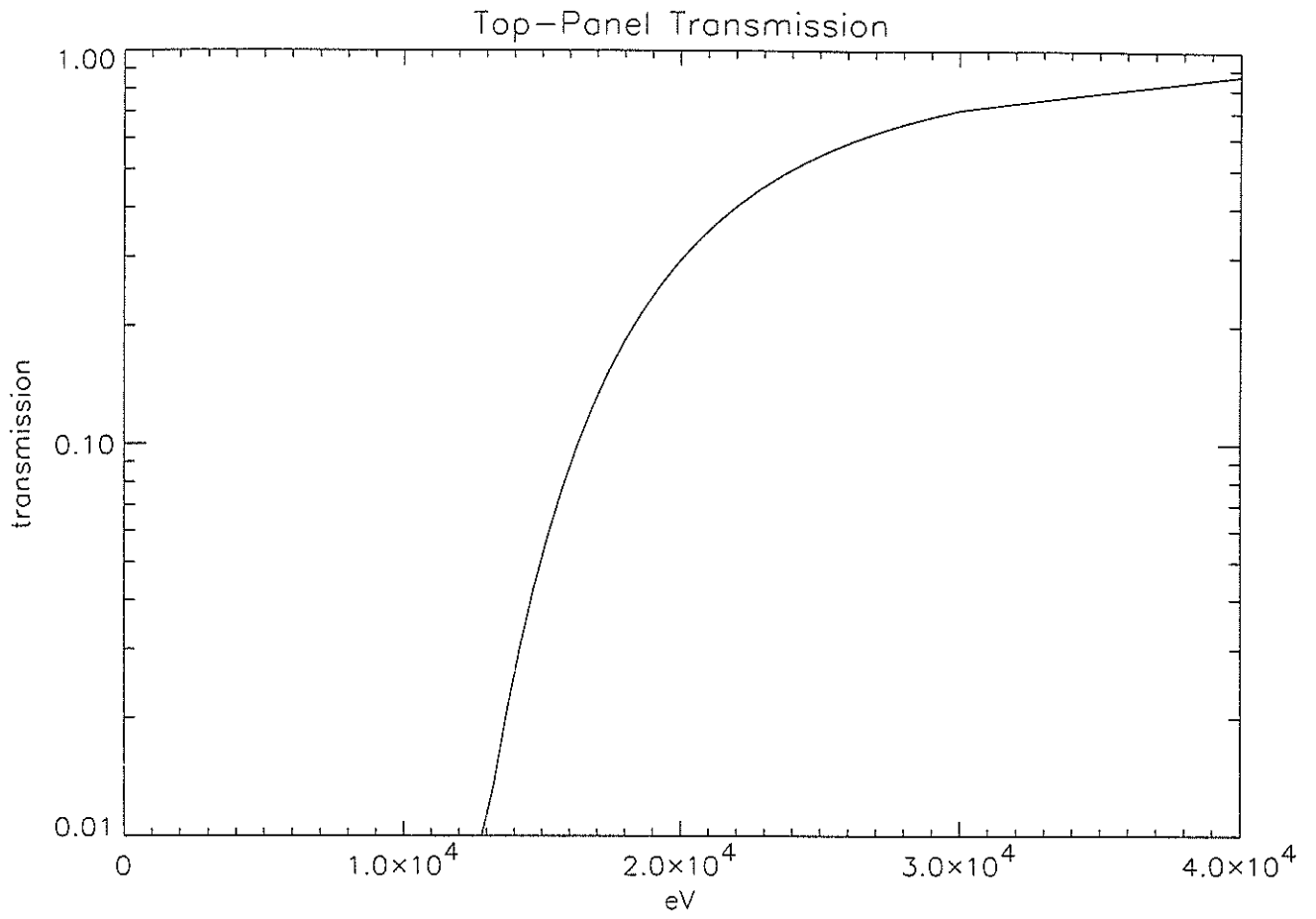
Figure 2: Transmission of X-rays through Top Panel
