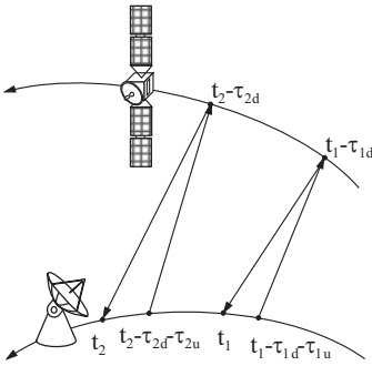
Fig. 6.11. The motion of the satellite and the ground station during signal travel time for two-way Doppler measurements
