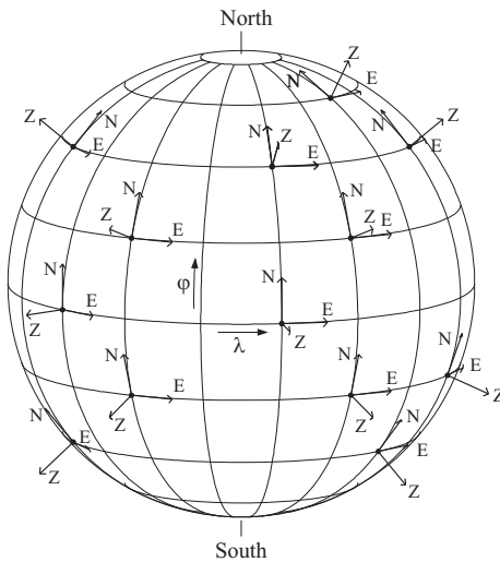
Fig. 6.7. Orientation of local horizontal coordinate systems
