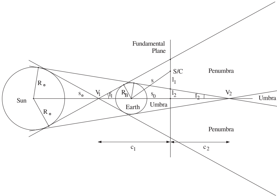
Fig. 3.7. Conical shadow model
