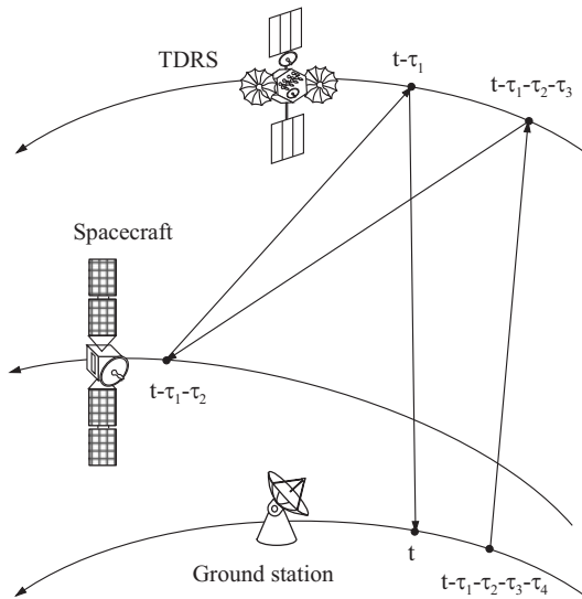
Fig. 9.10. Principle of TDRS four-way ranging measurements.
