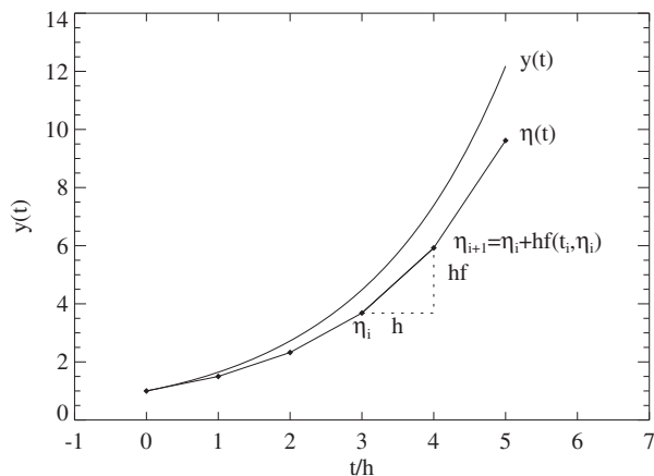
Fig. 4.1. Approximate solution of a differential equation \dot{\mathbf{y}} = \mathbf{f}(t, \mathbf{y}) using Euler steps of size h
