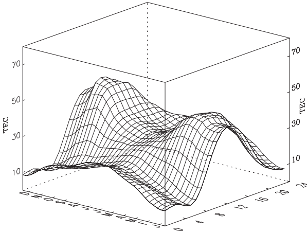
Fig. 6.14. Variation of the TEC with the time of the year and local time for a mid-latitude station based on the IRI 1995 model
