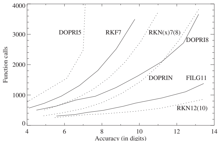
Fig. 4.2. Performance diagram of several embedded Runge-Kutta-Nyström methods for test case D1 ( e=0.1 ) of Hull et al. (1972). The number of function calls is plotted versus the accuracy in digits
