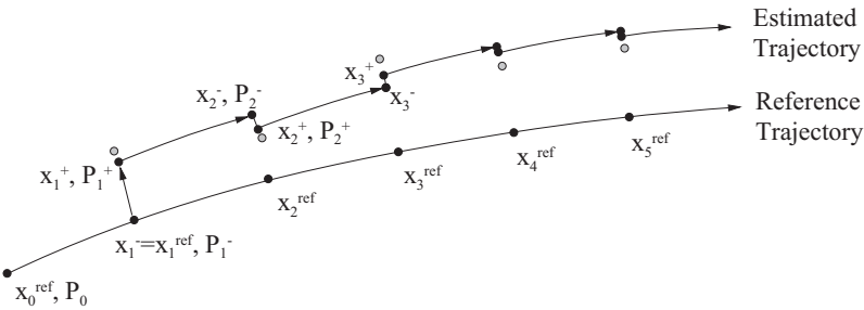
Fig. 8.7. The linearized Kalman filter (LKF) refers all measurements and state corrections to a common reference trajectory. Initially, when the covariance is still small, the filter output closely matches the observations (shaded circles). Later on, the filter approaches the true trajectory and becomes less sensitive to new data. Due to the increasing difference between the reference state and the estimated trajectory the filter output may become erroneous in case of non-linearities.
