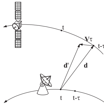
Fig. 6.6. The effect of aberration
