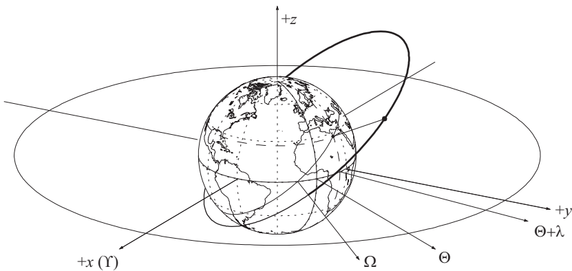
Fig. 2.8. The ground projection of a satellite orbit
