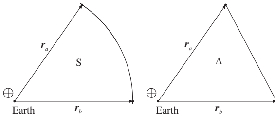
Fig. 2.14. Areas of sectors and triangles
