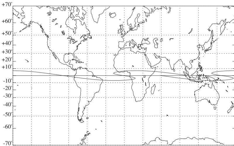
Fig. 2.10. Ground track of a sample geostationary transfer orbit ( a = 24\,400 km, e = 0.7307 , i = 7.0^\circ , T = 10^{\text{h}}5 )
