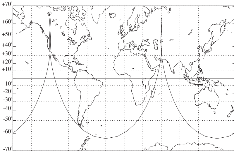
Fig. 2.11. 24 h ground track of a sample Molniya type orbit ( a = 26\,555 km, e = 0.7222 , i = 63.4^\circ , \omega = 270.0^\circ , T = 12^{\text{h}}0 )
