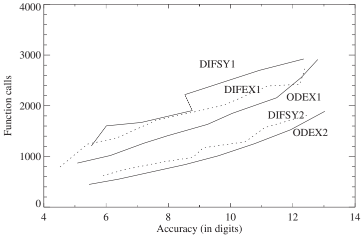
Fig. 4.8. Performance diagram of several extrapolation methods for test case D1 ( \epsilon=0.1 ) of Hull et al. (1972). The number of function calls is plotted versus the relative accuracy in digits. Note the jump in the graph for DIFSY1 that is caused by the stepsize and order control
