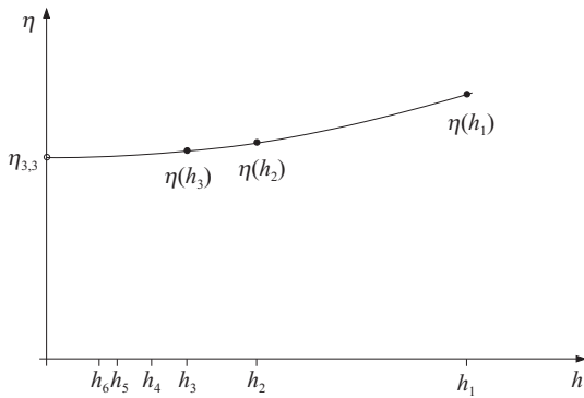
Fig. 4.7. Extrapolation of \eta(h) for h \rightarrow 0 .
