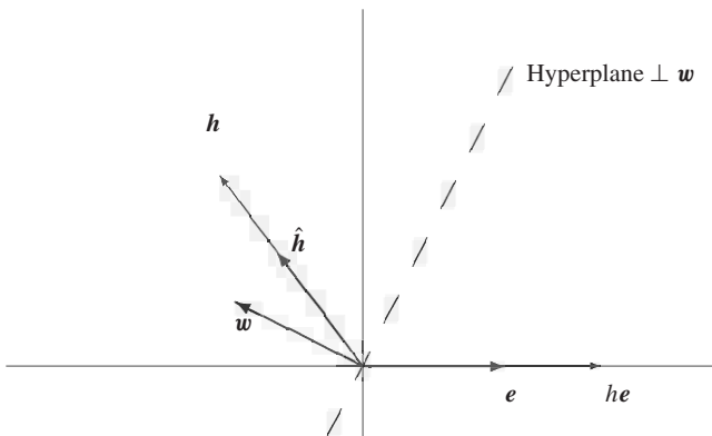
Fig. 8.4. Householder Transformation
