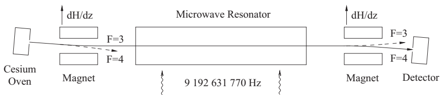
Fig. 5.2. Schematic view of a cesium-beam atomic clock
