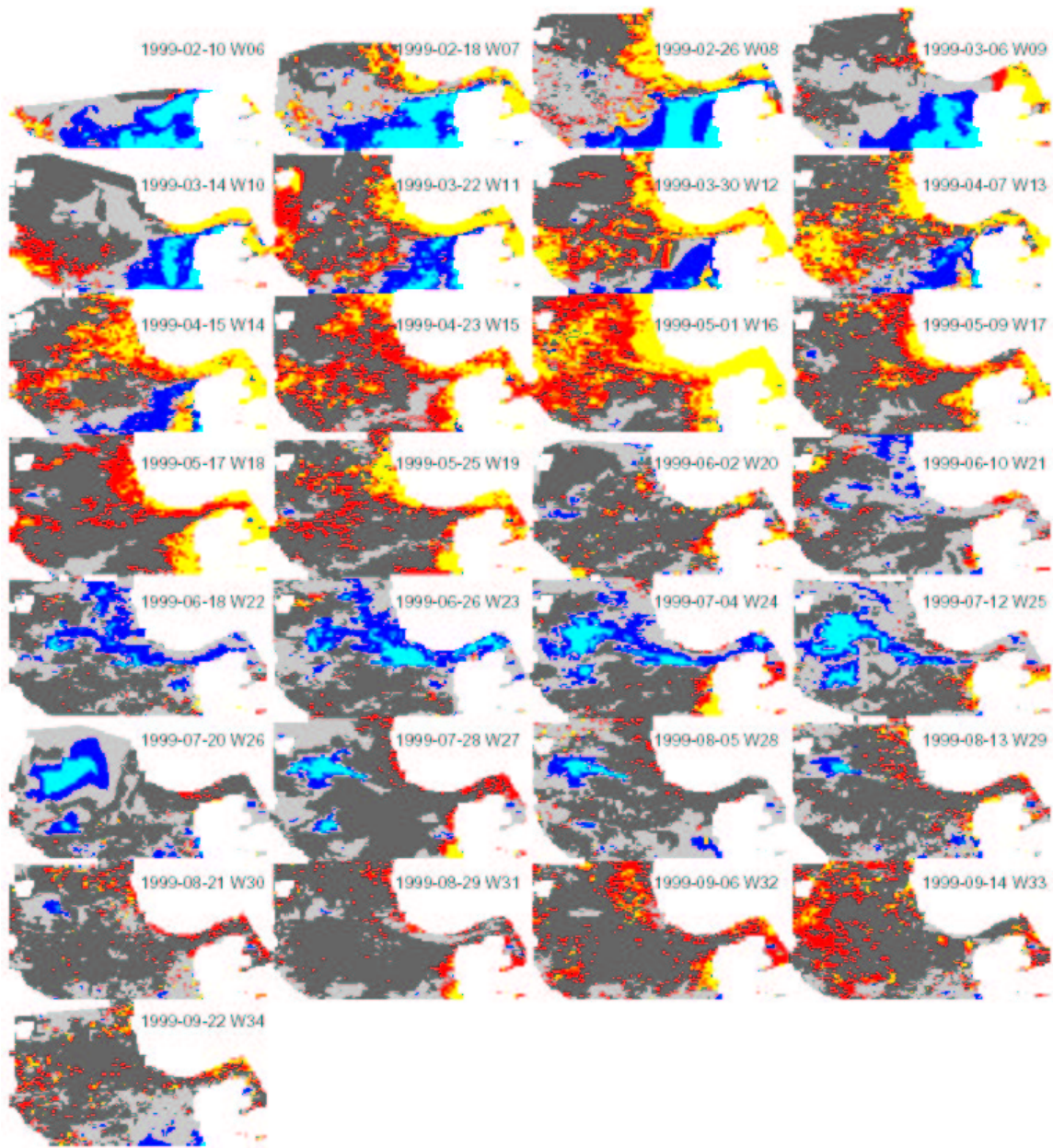
Figure 16: Classified water masses based on SeaWiFS constituents.
