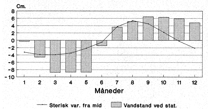
Figure 10: Computed steric effect at the lightship Anholt Syd averaged over 100 years, along with the actual sea level observations on a monthly base.
