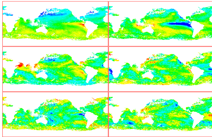
Figure 12: SST, linear canonical variates 1-6 row-wise.
