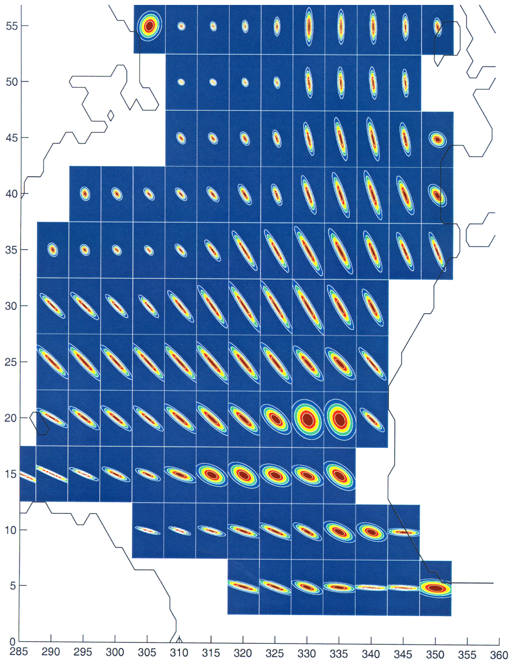
Figure 4: Fitted zonal-temporal autocorrelation models derived from TOPEX/POSEIDON observations in the North Atlantic. The small squares represent spatial lags from -500 to 500 km (x-axis) and temporal lags from -200 to 200 days (y-axis). Contour interval is 0.1 and red indicate high correlations above 0.9 .
