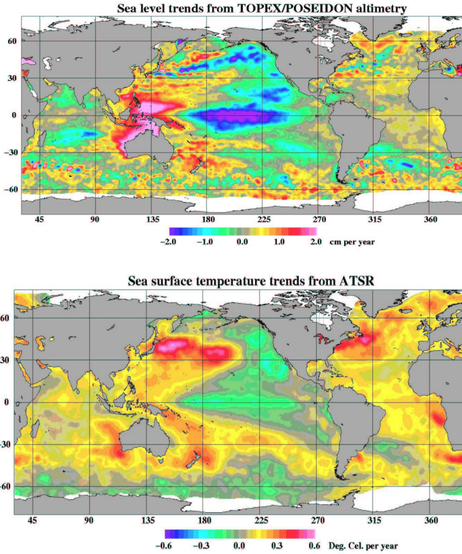
Figure 21: Global sea level and sea surface temperature eight-year trends estimated from TOPEX/POSEIDON altimetry and ATSR (ERS 1+2).
