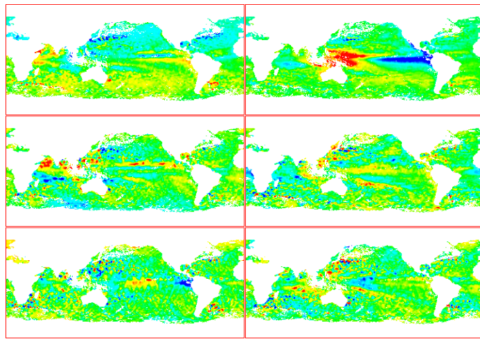
Figure 13: SSH, linear canonical variates 1-6 row-wise.
